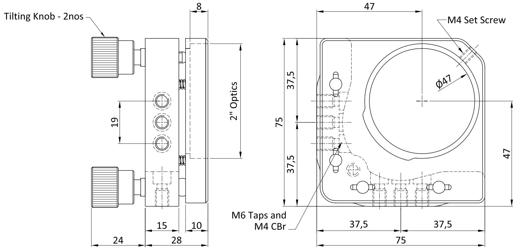
2" or 50mm optic mount
