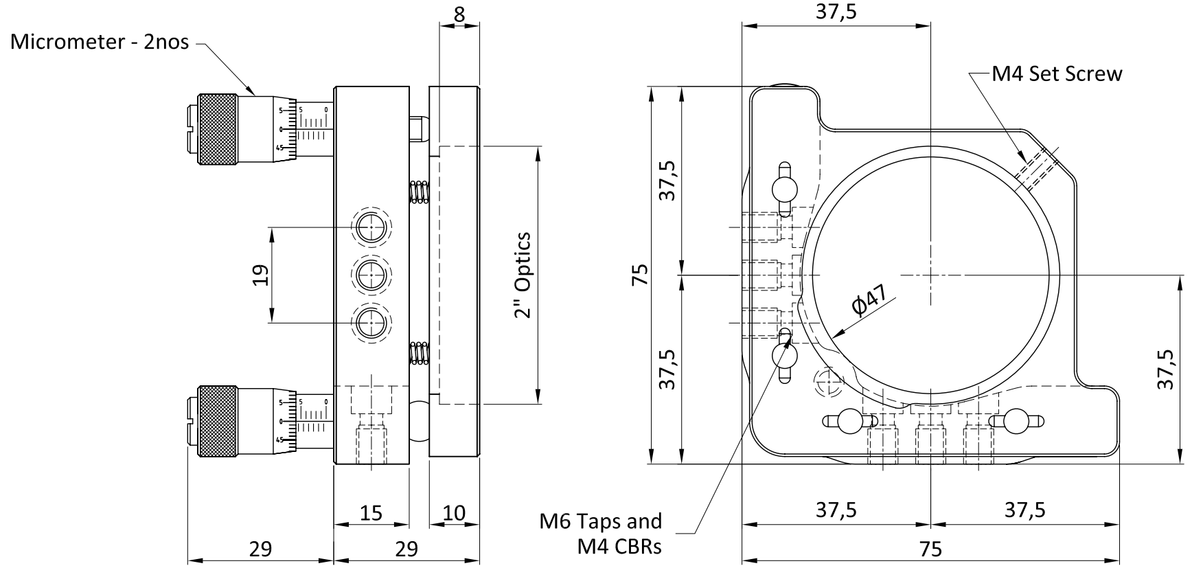
2" or 50mm optic mount
