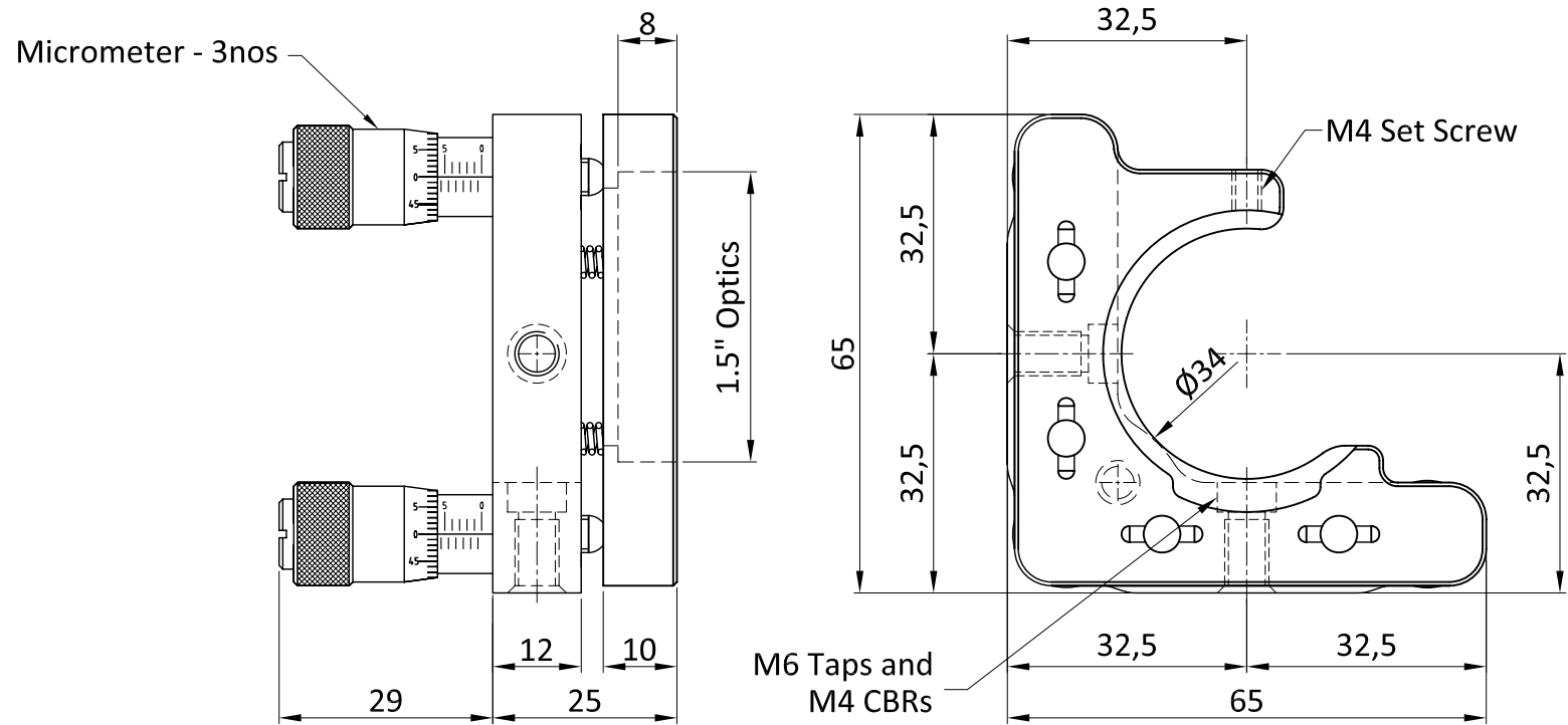
1.5" or 38mm optic mount
