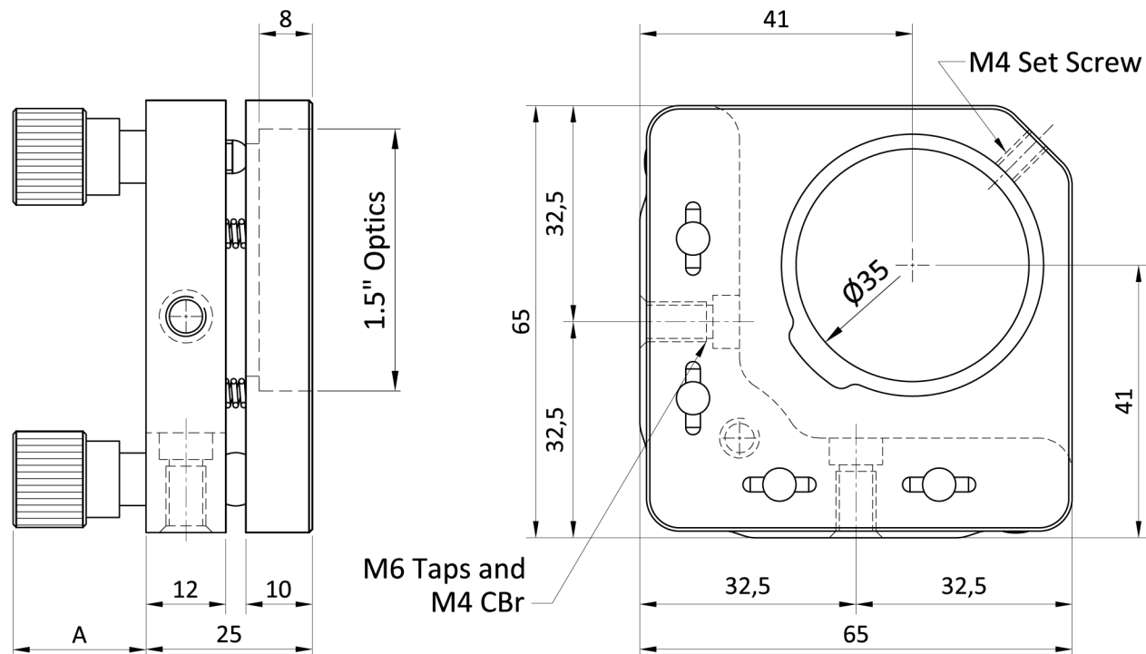
1.5" or 38mm optic mount
