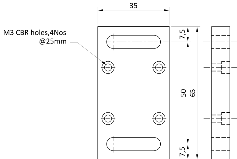
BASE PLATE
