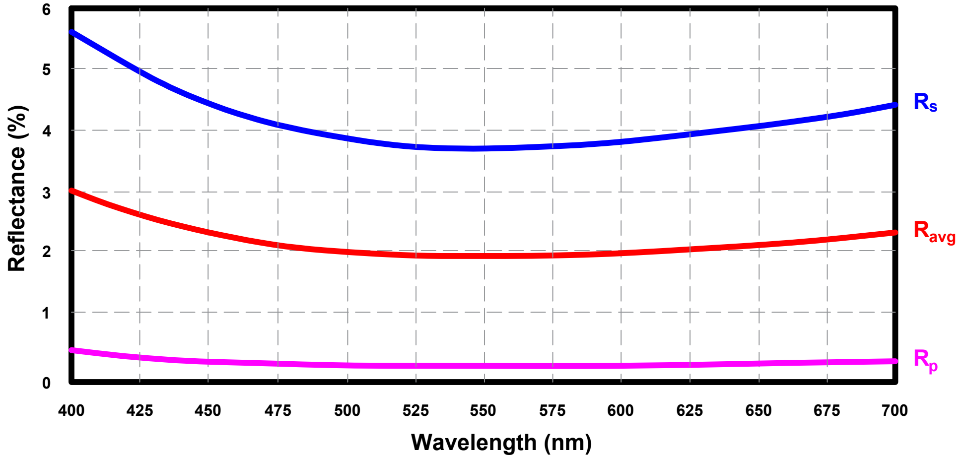
Single Layer MgF2: Wavelength vs Reflectance (45° AOI)
